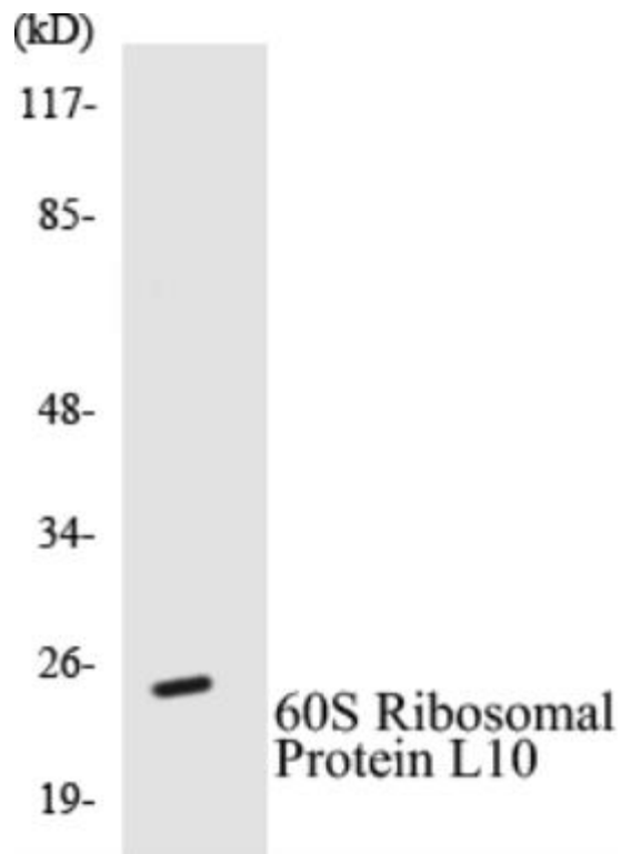
Figure 1. Anti-60S Ribosomal Protein L10
