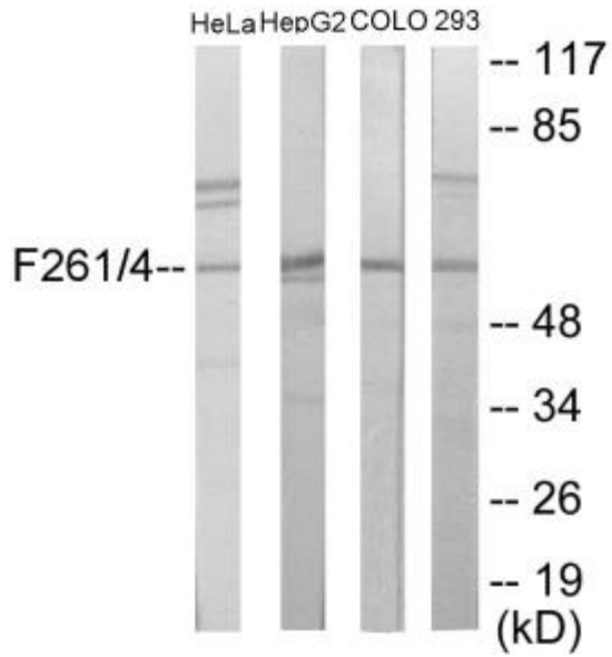
Figure 1. Anti-PFKFB1/4
