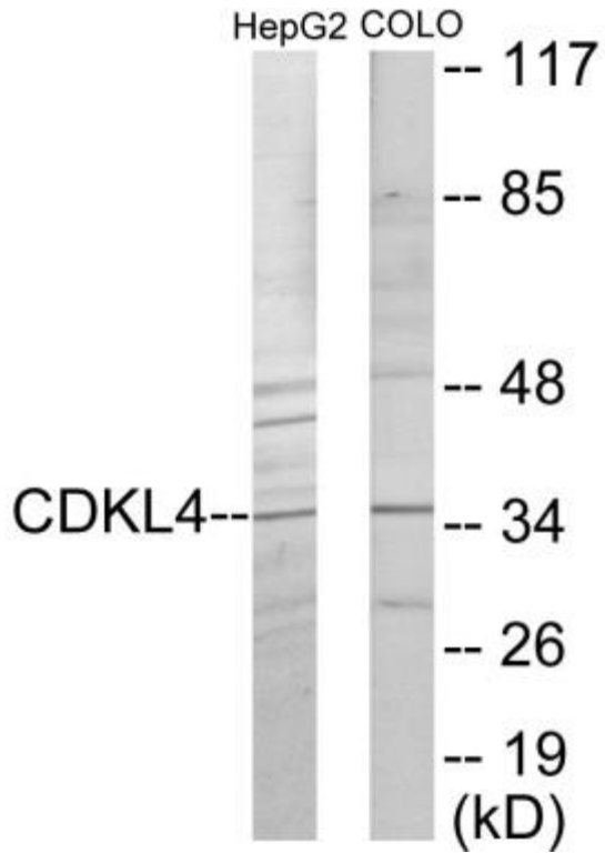
Figure 1. Anti-CDKL4
