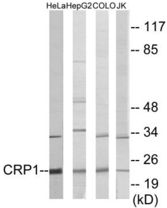
Figure 1. Anti-CRP1
